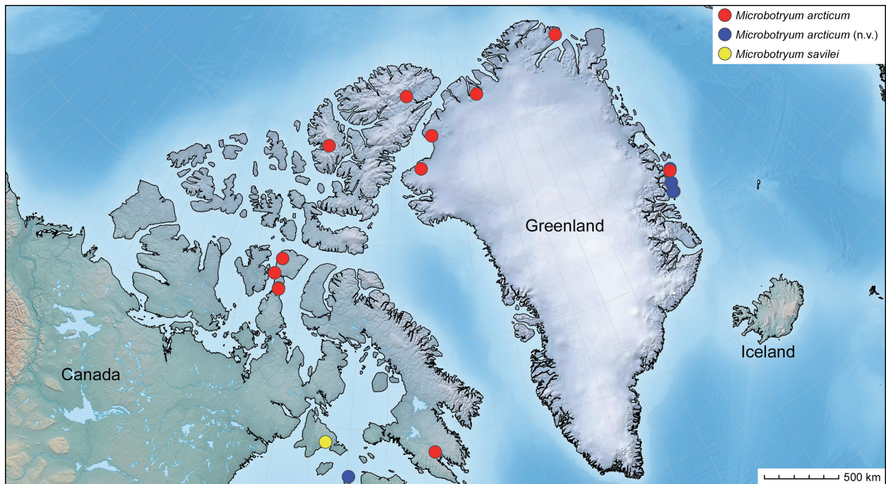
Fig. 5. Geographic distribution of Microbotryum arcticum and M. savilei (generated with SimpleMapper, Shorthouse 2010).
