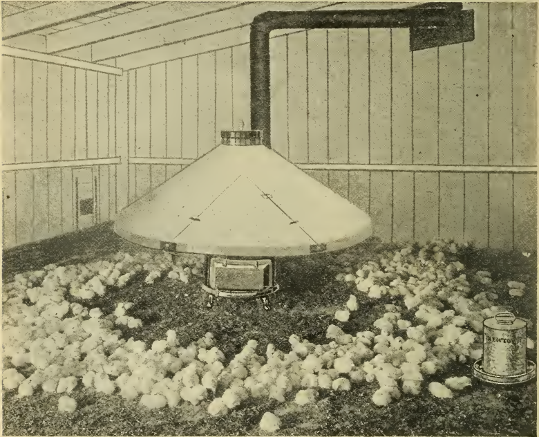
FIG. 168A.—A modern coal-burning brooder stove. Note the contented, quiet condition of the chicks and the large size of the house. (Photo Newtown Inc. and Brooder Co.)
