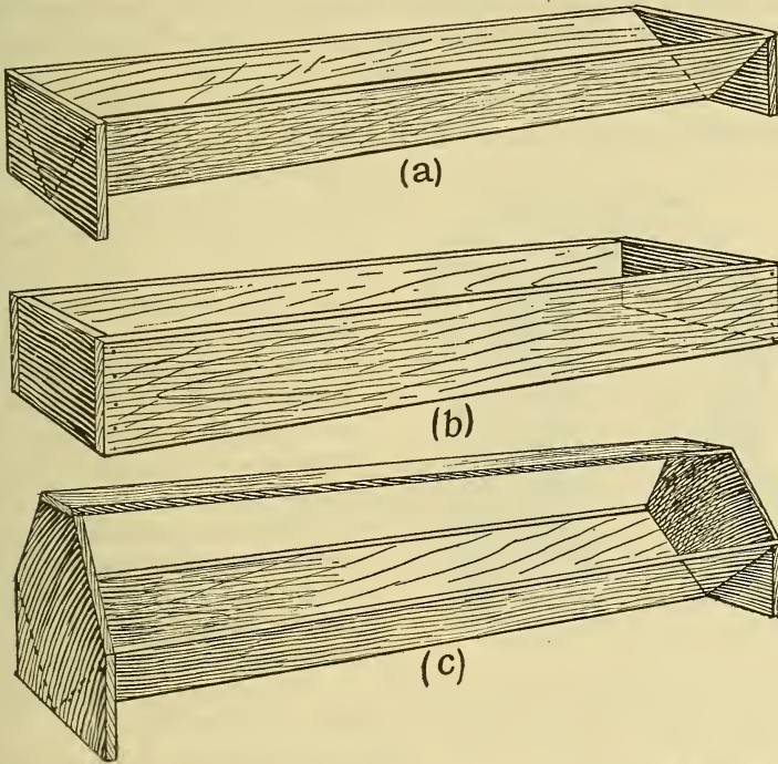
FIG. 101.—Common types of feeding troughs. a, Open V-shaped; b, square form; c, V-shaped, covered.
