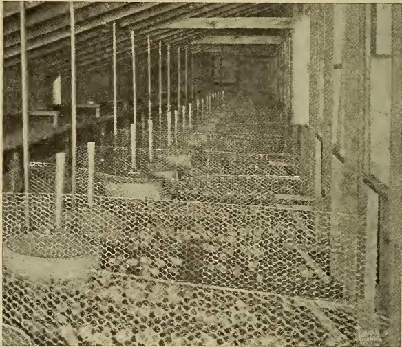
FIG. 165.—Portable indoor hovers make it possible to use the laying houses for brooding purposes. (Photo by Rancoeas Poultry Farm.)
