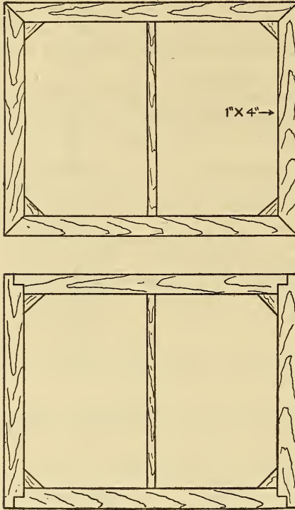
FIG. 78.—Two plans for constructing frames for muslin curtains.
