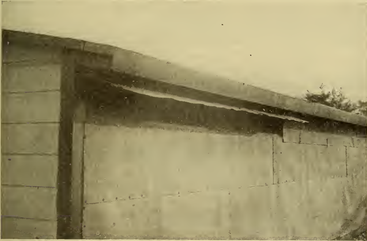
FIG. 67.—An efficient rear ventilator for summer use. It allows the air to enter the back of the house, and circulate between the sheathing and the roof, cooling the roosting quarters on summer nights. This is most valuable for shed-roofed houses that are covered with paper. Cornell University was the first Experiment Station to recommend back ventilation for the poultry house.
