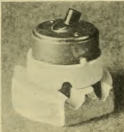
FIG. 238.—A G. E. tumble switch used in connection with alarm clocks. As the alarm goes off the winding stem turns and pushes the ball switch over.
