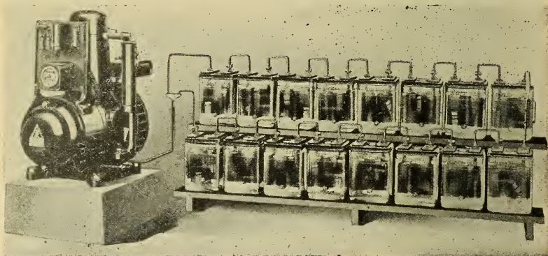
FIG. 235.—A farm unit electric lighting plant just suited to light the home and the poultry houses. (Photo Delco Lighting Corporation.)
