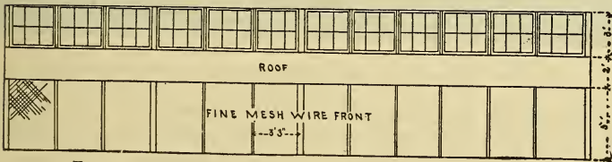
Fig. 91a.—Half-monitor type of laying house; Working plans.
