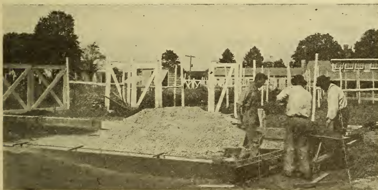
FIG. 82.—Placing fresh concrete in completed forms for foundation wall.
