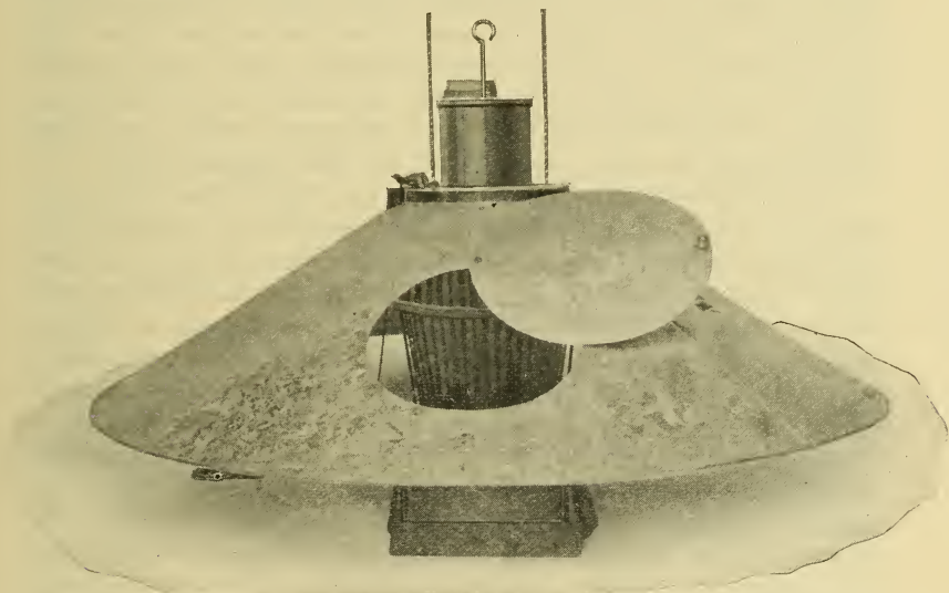
FIG. 168B.—The smaller type of coal-burning brooder stove which is suited for a house about 10 by 12 feet and can readily handle around 300 chicks. (Photo United Brooder Co.)
