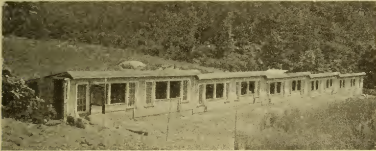
FIG. 85.—Five double unit sections of the N. J. Multiple Unit Laying House. Built in steps to conform to slope of land. Note the arrangement of windows for light and ventilation; also the drip or roof projection over the front to keep out driving storms.
